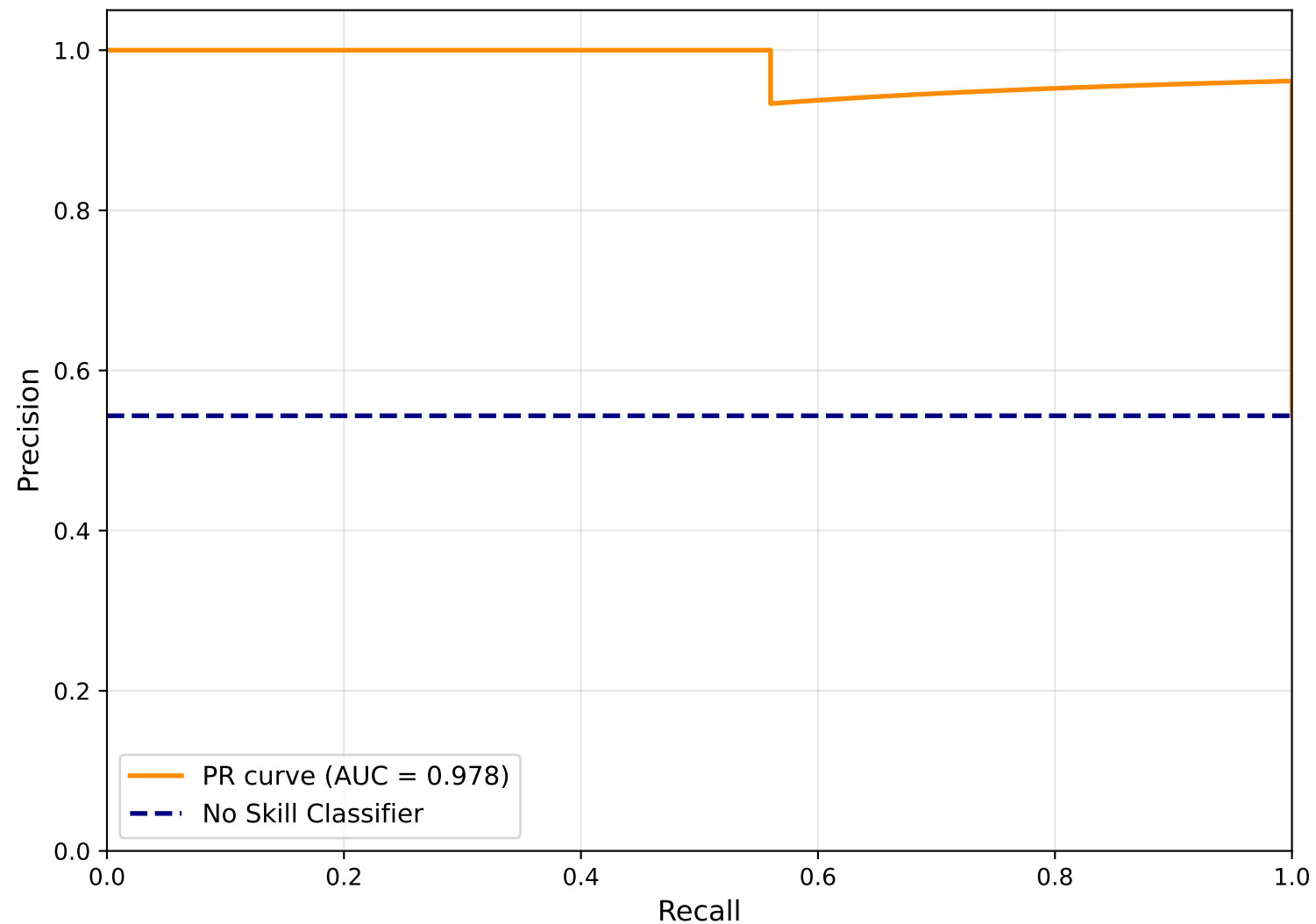
Precision-Recall Curve for Tuned CatBoost
